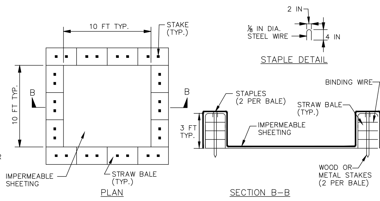
PLAN WASHOUT STRUCTURE WITH STRAW BALES
