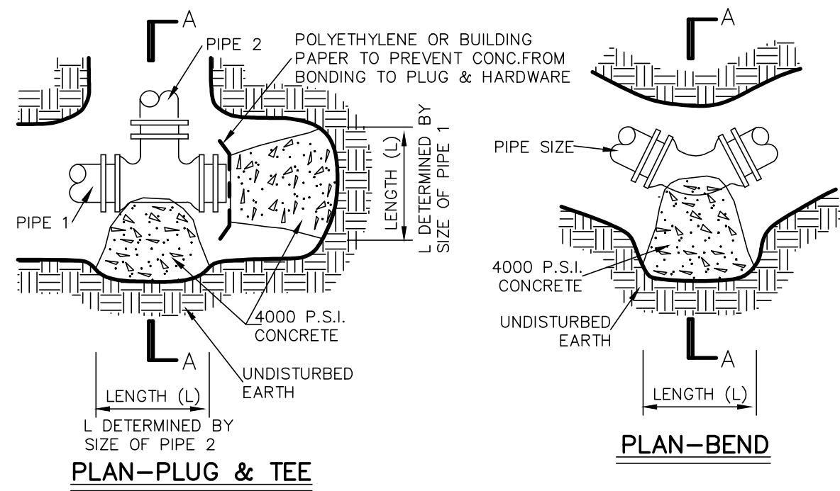
PLAN-PLUG & TEE
