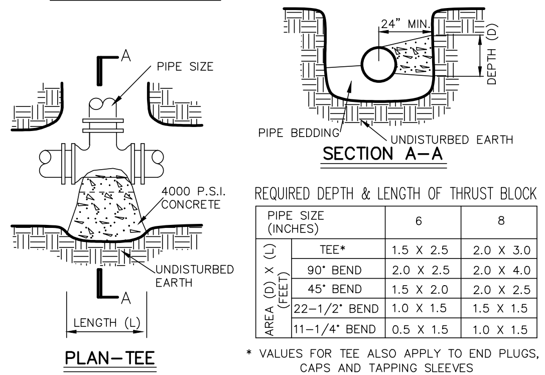
THRUST BLOCK DETAILS NOT TO SCALE
