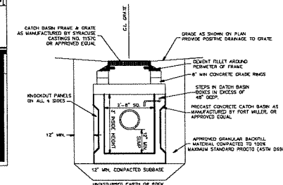
CATCH BASIN DETAIL NOT TO SCALE
