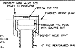
MONITORING WELL DETAIL NOT TO SCALE
