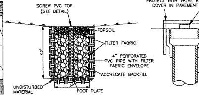
MONITORING WELL DETAIL NOT TO SCALE
