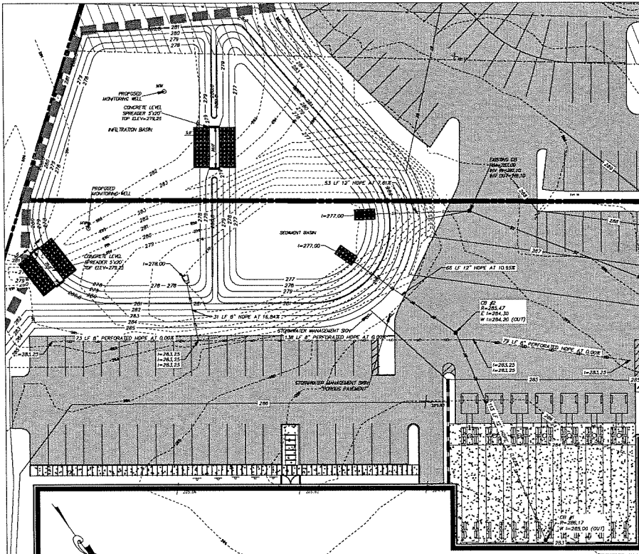
STORM SEWER PLAN SCALE: 1"=30'
